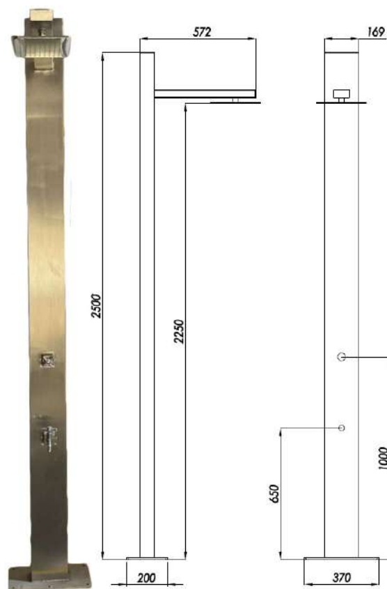
STAINLESS SQUARE SHOWER SYSTEM
