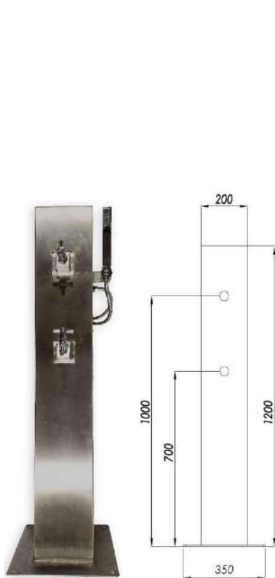
STAINLESS SHORT SHOWER SYSTEM
